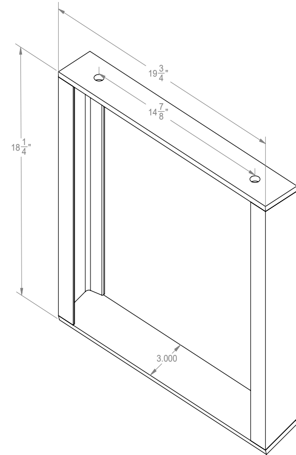
P/N 100897 Ladder Ramp Long Leg Assembly
