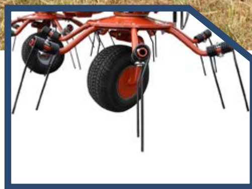
Like all TT Series Tedders, the TT6101 features tubular tine arms. Tubular arms provide extra durability in the field. A shot-peened double tine slides over the arm for easy install.
