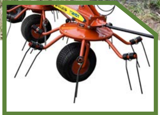
Like all TT Series Tedders, the TT4101 features tubular tine arms. Tubular arms provide extra durability in the field. A shot-peened double tine slides over the arm for easy installation.
