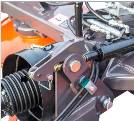
Hydraulic Tilt (Optional Feature)
